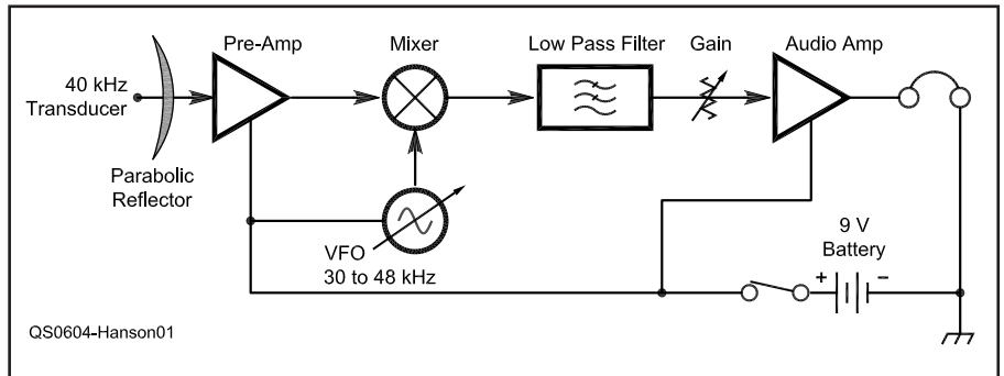
Figure 1 — Simplified block diagram of the ultrasonic detector.
