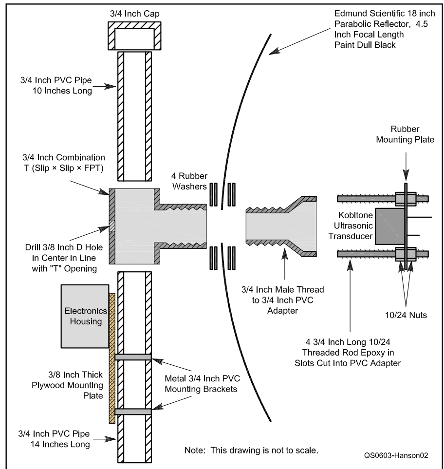
Figure 2 — Ultrasonic dish assembly.
